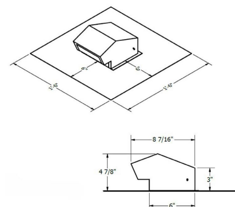
BATHROOM/DRYER VENT
