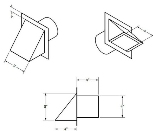
4" WALL VENT
