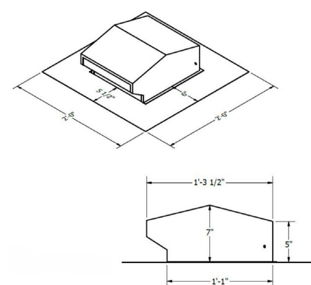
RANGE VENT
